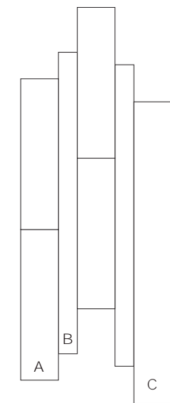
MOSAICO 23 ○ 300 X 600 mm A 75 X 300 B 37.5 X 600 C 75 X 600 ○ matte surface
