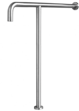
GB-T32-7-7 Safety Grab Bar Material SUS 304 Stainless Steel Thickness 700x700mm OD:32mm 304
