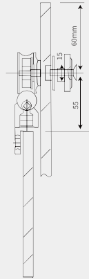
Setional installation diagram
