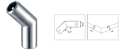
EPGC-006-135° Rod to Glass connector
