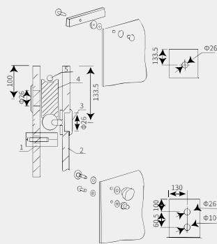
Sectional installation diagram Φ25 pipe bathroom hanging wheel
