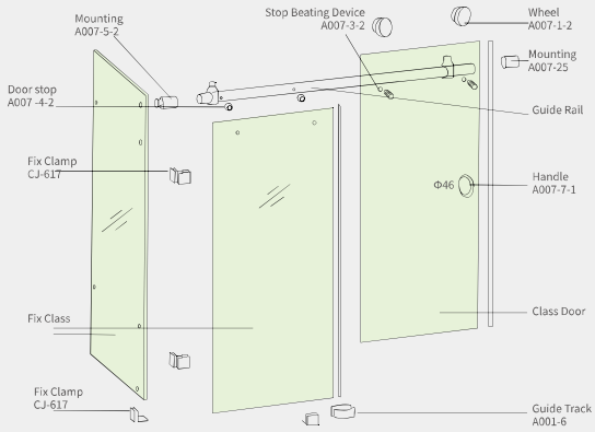
Plane installation diagram
