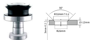
Countersunk holes from the front side
