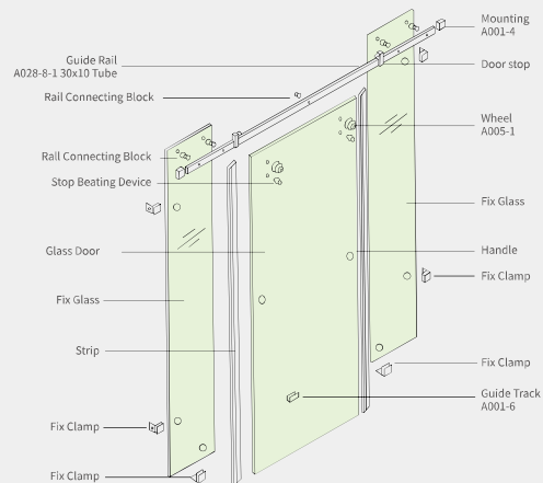
Plane installation diagram
