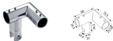
EPGC-004-F90 Rod to Glass connector
