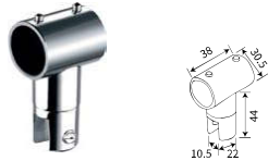
EPGC-002-A Rod to Glass connector
