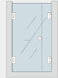
Installation Pattern C
