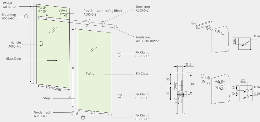
Plane installation diagram
