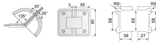
SD-135B 135° 斜边
