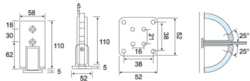
SD-033 90° 双边长夹
