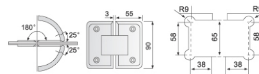
SD-180C 180° 斜边
