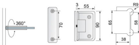
SD-9002 360° 斜边
