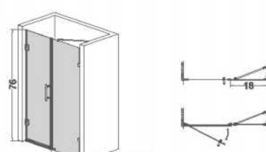
with 18" stationary side panel
