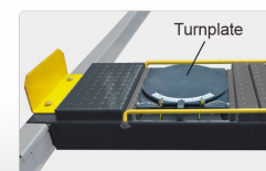
Optional Turnplate, Kits No. 40101. Each alignment lift need 2 units. Only for the model A465A A465AE
