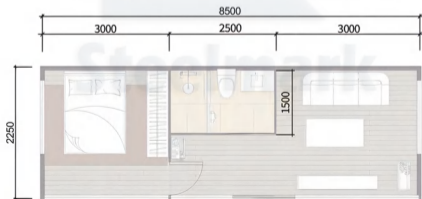
Floor Plan
