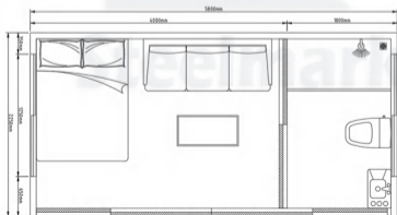
Floor Plan
